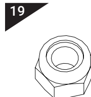
x4 45001521 Nylock Nut M8
